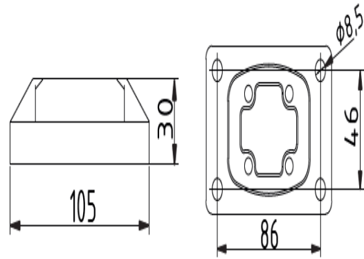
DRAWING
